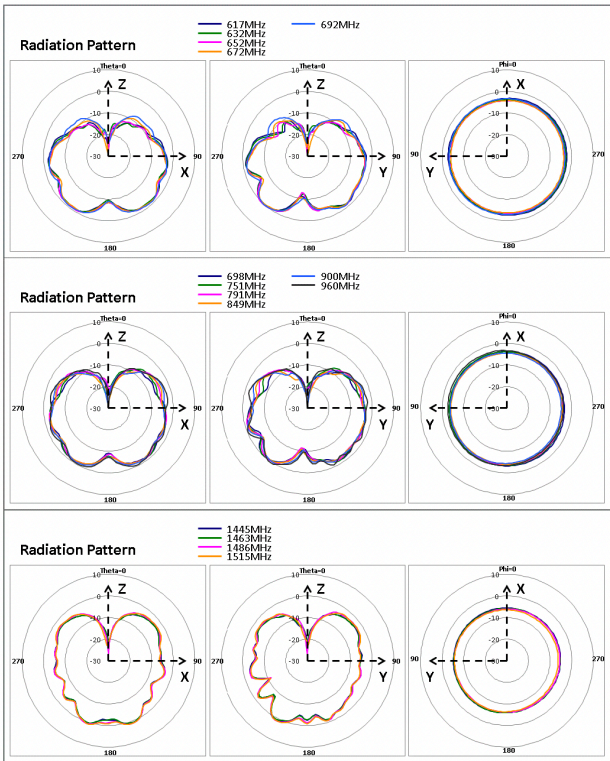
Radiation pattern
